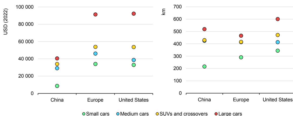
Figure 1.7 Sales-weighted average retail price (left) and driving range (right) of BEV passenger cars in selected countries, by size, in 2022
